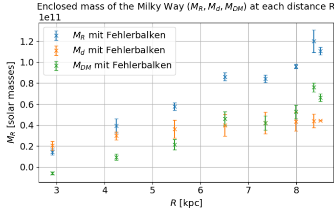
Figure 12: The enclosed mass of the milky way at each distance R broken down for the differnt mass distributions with M_R being the total enclosed mass, M_d being the enclosed baryonic mass and M_{DM} being the enclosed mass of the dark matter.
