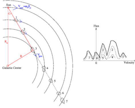
Figure 1: A schematic representation of the rotation of H1 clouds around the galactic centre together with the resulting line profile to the right [2].
